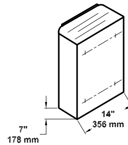
Side / Back / Top View
